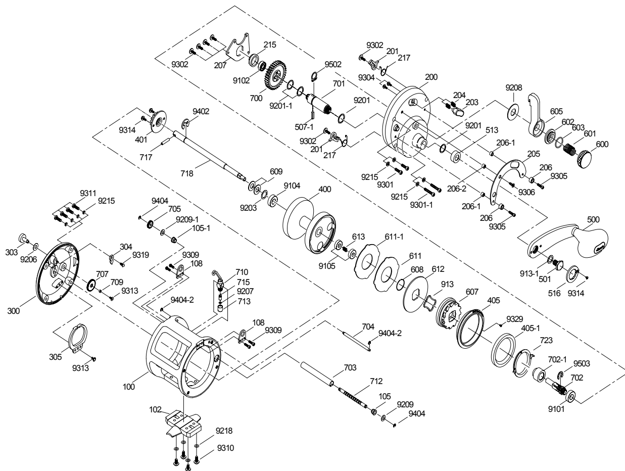
TG - 15L (1 of 2) Spare Parts
